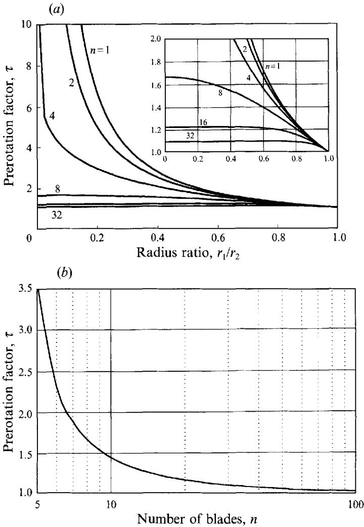
FIGURE 9. Prerotation factor for pump impellers fitted with straight radial blades: (a) exact value; (b) asymptotic solution as \mu^{1/2} \rightarrow 0 .
