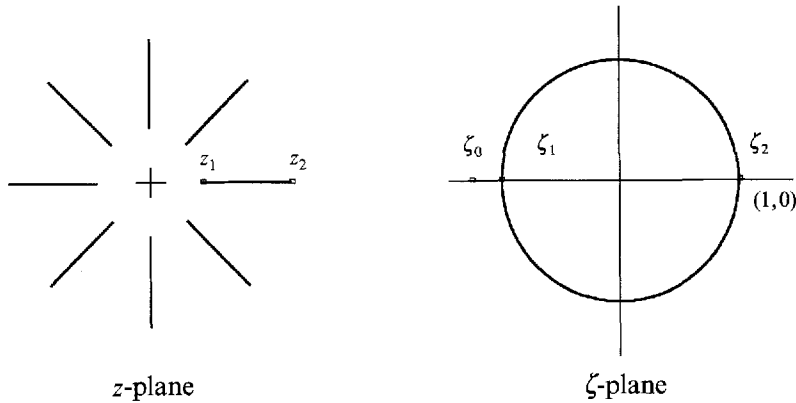
FIGURE 2. Mapping of eight straight radial blades.
