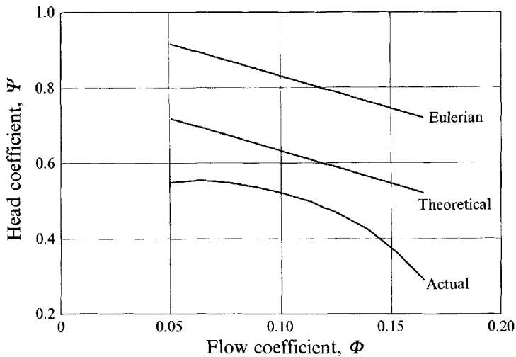
FIGURE 12. Head characteristic for 60^\circ , logarithmically bladed pump impeller with eight blades, having 100 mm outer radius, and receiving zero prerotation.
