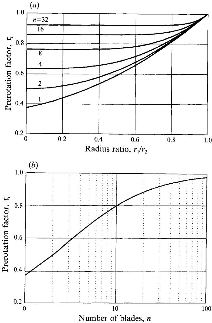
FIGURE 19. Prerotation factor for radially bladed turbine impellers: (a) exact value; (b) asymptotic solution as \mu^2 \rightarrow 0 . Note that the values for \tau_i at r_1/r_2 = 0 , given in (a), are equal to the values of \tau_i in (b).
