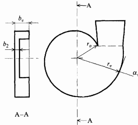
FIGURE 14. Logarithmically curved volute.
