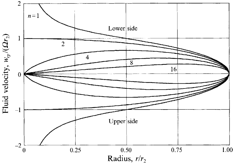
FIGURE 6. Displacement-flow fluid velocity along straight radial blades as \mu > 0 .
